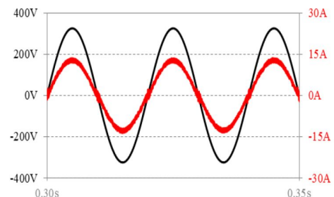
Figure 4: Simulation results: voltage and current in the electrical power grid during the charging process (G2V).
