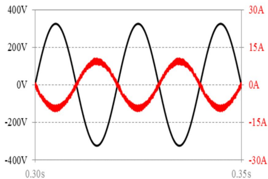
Figure 5: Simulation results: voltage and current in the electrical power grid during the discharging process (V2G).
